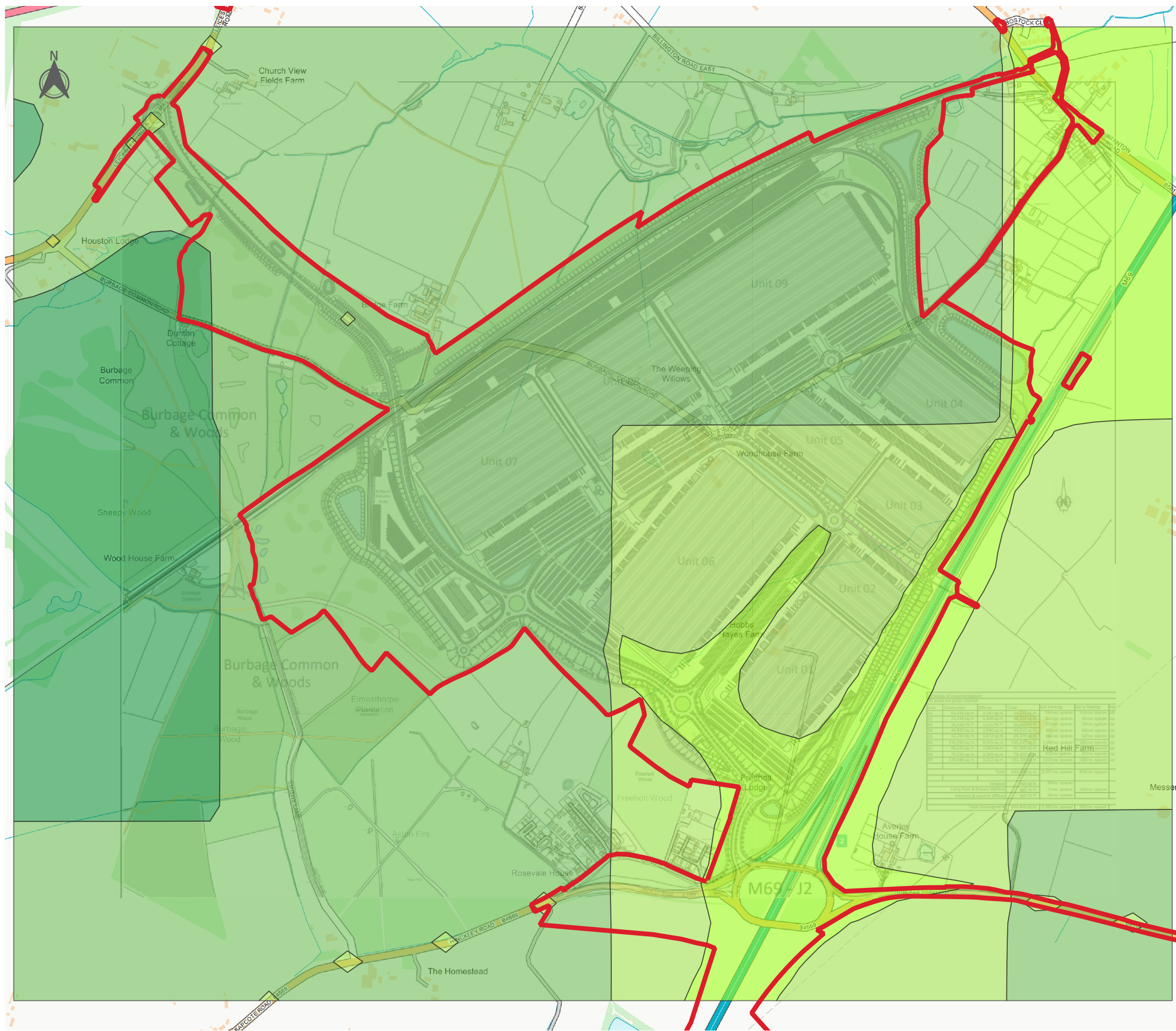
ES Figure 9.27 - Operational Phase Road Traffic Emissions - Main HNRFI Site Annual Mean PM 2.5 Concentrations - Opening Year
